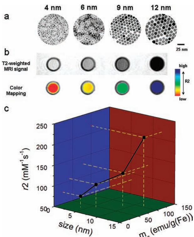
FIGURE 9. Nanoscale size effects of MEIO nanoparticles on MR contrast effects: (a) TEM images; (b) MR images and their color maps; (c) plot of m_s and r_2 values vs. size of 4, 6, 9, and 12 nm MEIO. Reproduced with permission from ref 13. Copyright 2005 American Chemical Society.
