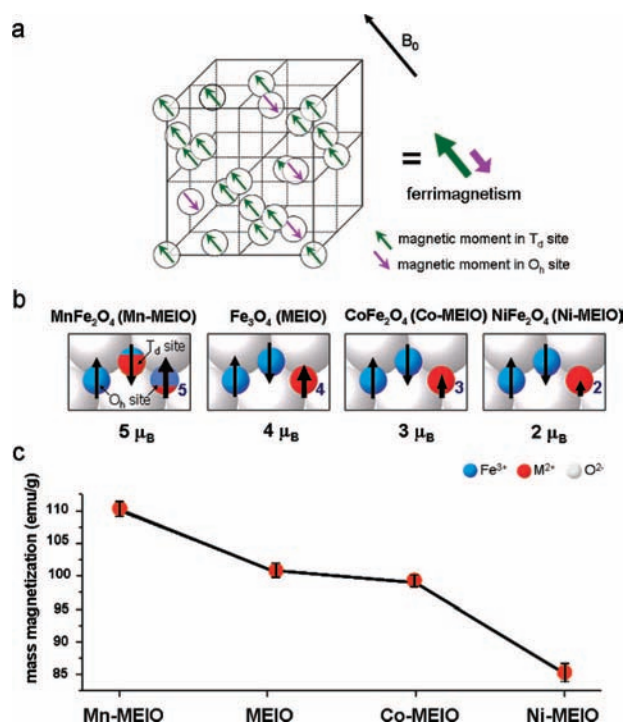
FIGURE 8. (a) Ferrimagnetic spin structure of inverse spinel ferrites and (b) schematic spin moments and (c) mass magnetization values of various metal-doped MEIO nanoparticles ( \text{MFe}_2\text{O}_4 , \text{M} = \text{Mn, Fe, Co, Ni} ). Reprinted with permission from Nature Medicine (www.nature.com), ref 14. Copyright 2007 Nature Publishing Group.
